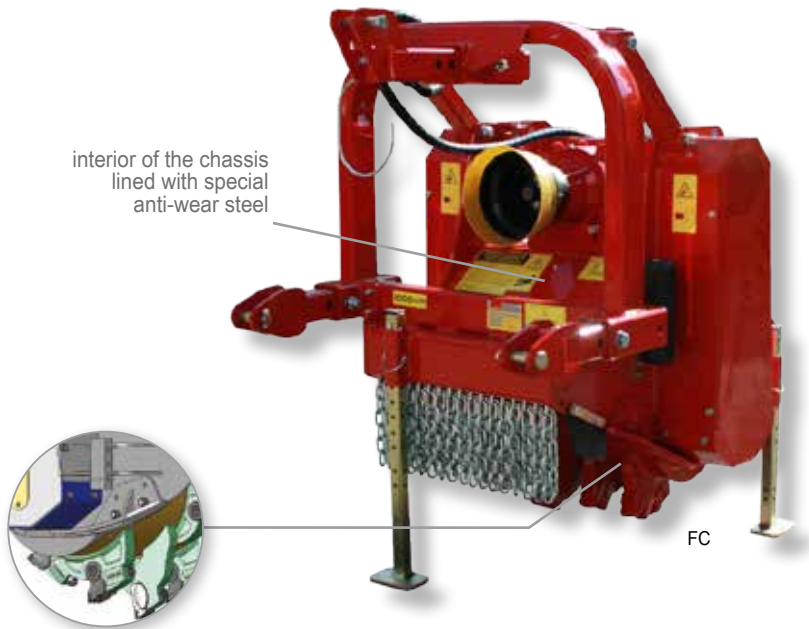
- skids adjustable in height - exposed rotor for tilling the soil
