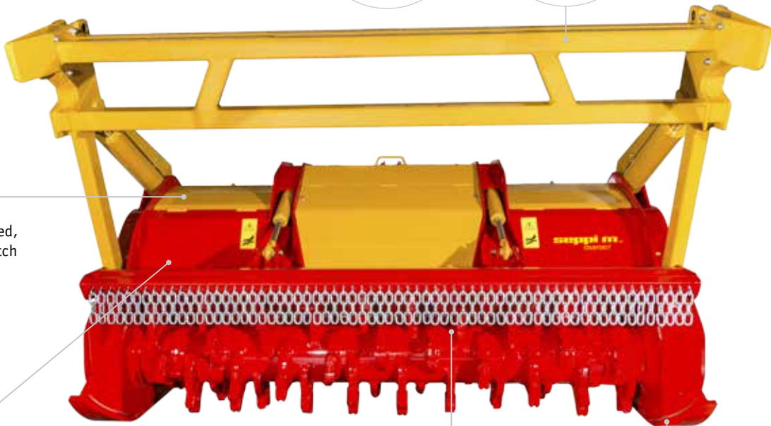
Guard frame for felling operations and to protect the tractor (option)
