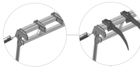
Guard frame for felling operations and to protect the tractor (option)
